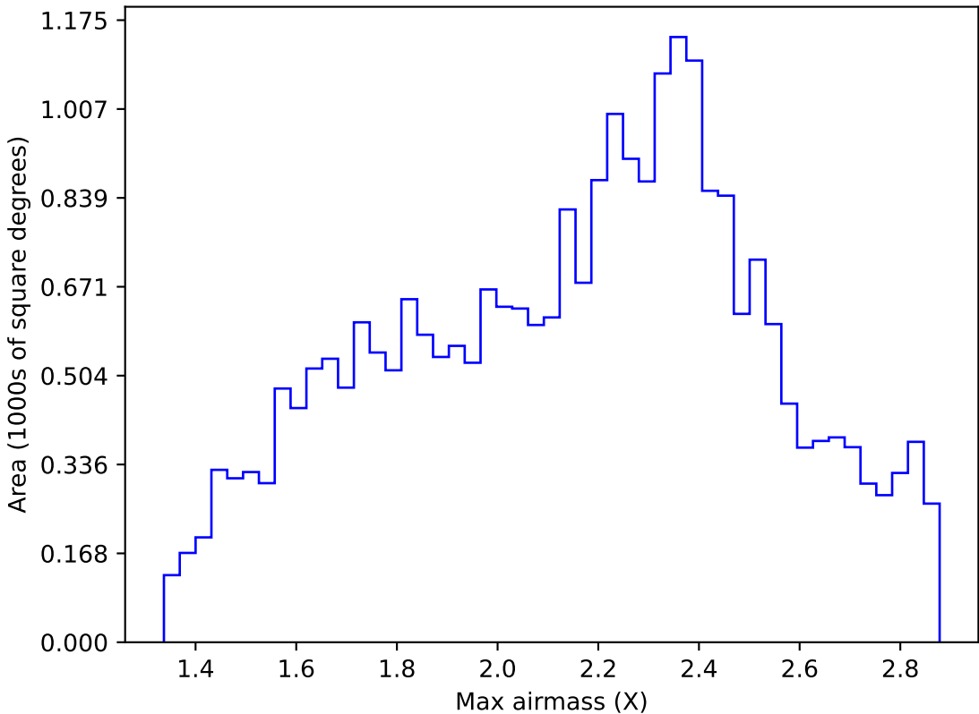
too_elab_r8_d2_ugrizy_v3.4_10yrs Yr 1 all bands: Max airmass
