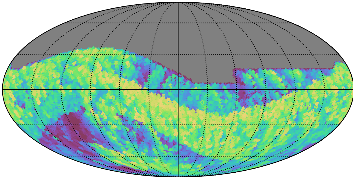
too_elab_r8_d2_ugrizy_v3.4_10yrs All sky z band: Max airmass
