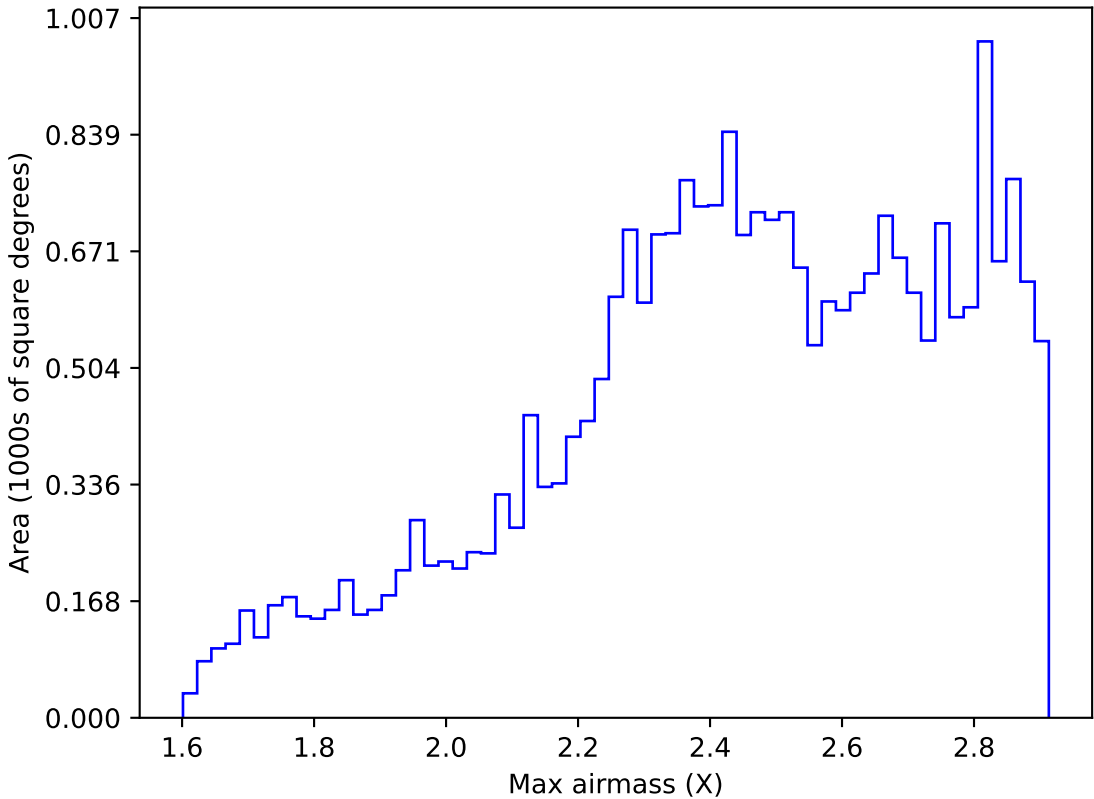
too_elab_r8_d2_ugrizy_v3.4_10yrs All sky z band: Max airmass
