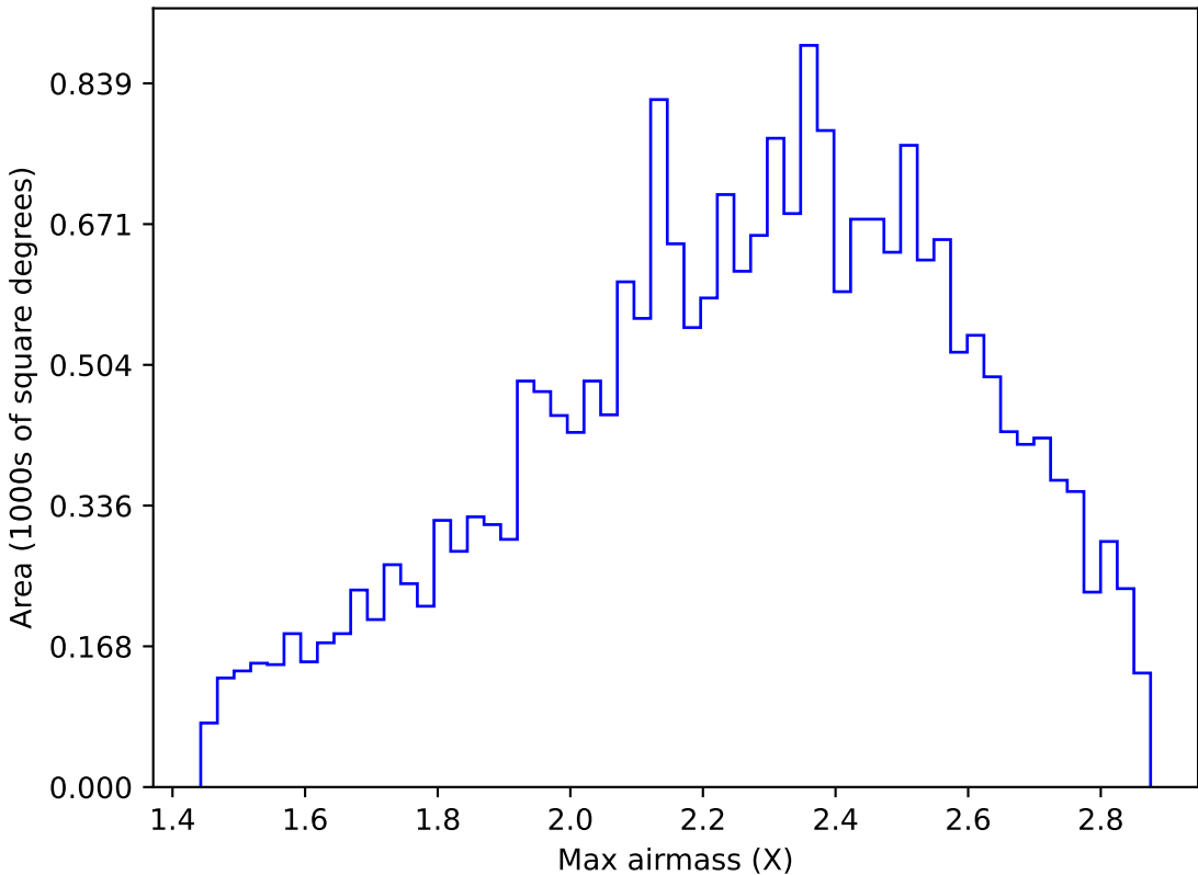
too_elab_r8_d2_ugrizy_v3.4_10yrs All sky y band: Max airmass
