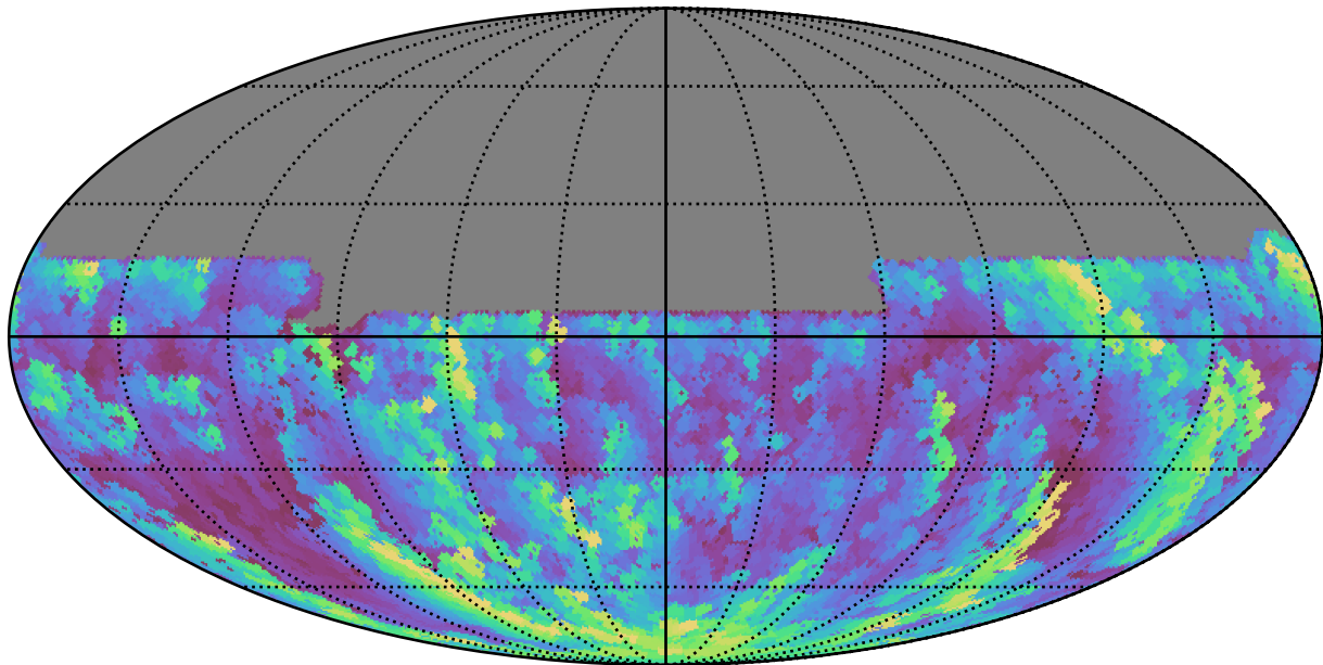
too_elab_r8_d2_ugrizy_v3.4_10yrs All sky u band: Max airmass
