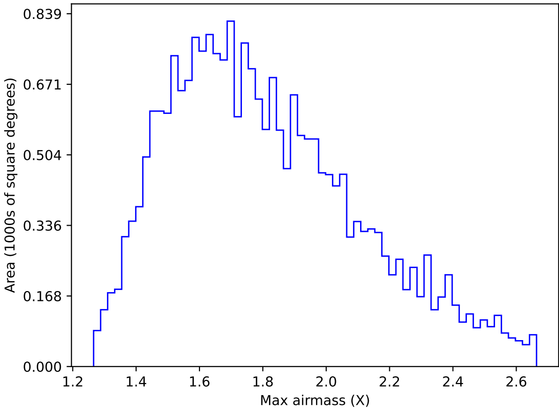
too_elab_r8_d2_ugrizy_v3.4_10yrs All sky u band: Max airmass
