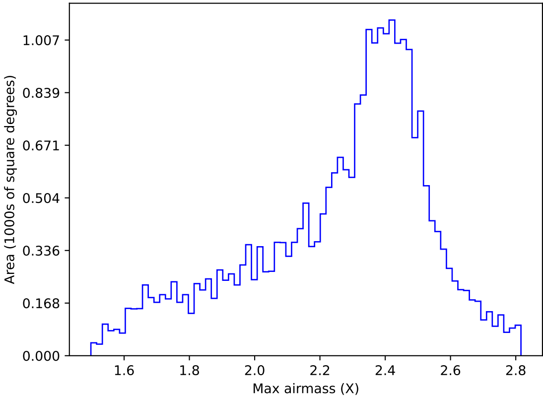
too_elab_r8_d2_ugrizy_v3.4_10yrs All sky r band: Max airmass
