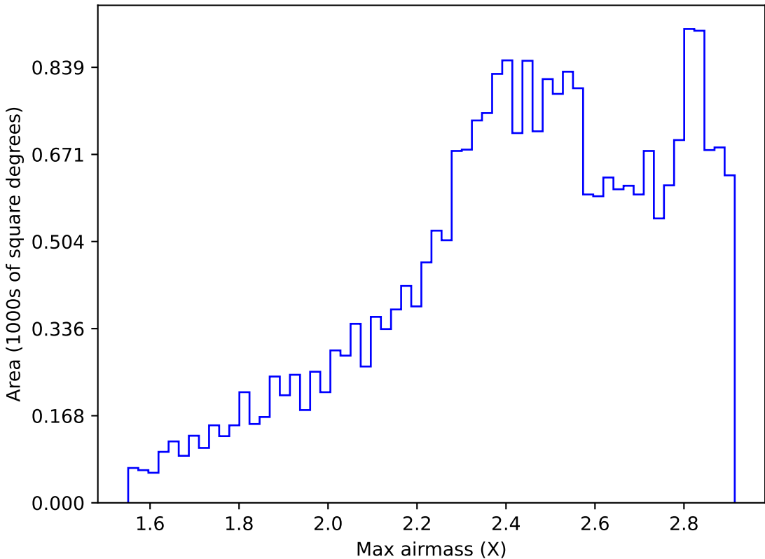
too_elab_r8_d2_ugrizy_v3.4_10yrs All sky i band: Max airmass
