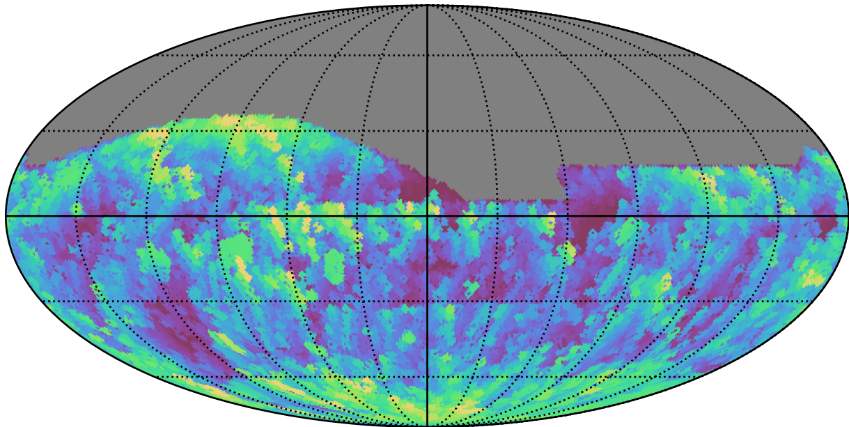
too_elab_r8_d2_ugrizy_v3.4_10yrs All sky g band: Max airmass
