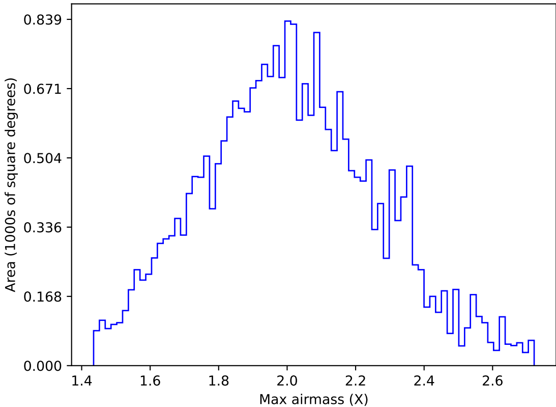
too_elab_r8_d2_ugrizy_v3.4_10yrs All sky g band: Max airmass
