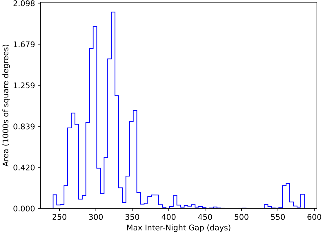
too_elab_r8_d2_ugrizy_v3.4_10yrs WFD y band: Max Inter-Night Gap
