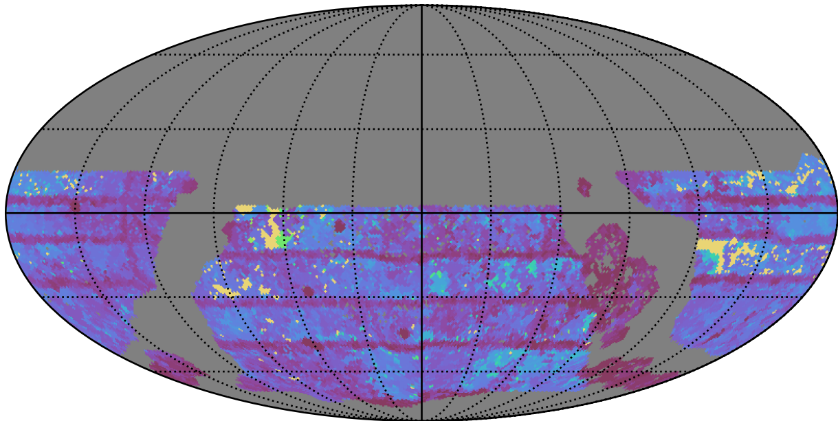
too_elab_r8_d2_ugrizy_v3.4_10yrs WFD r band: Max Inter-Night Gap
