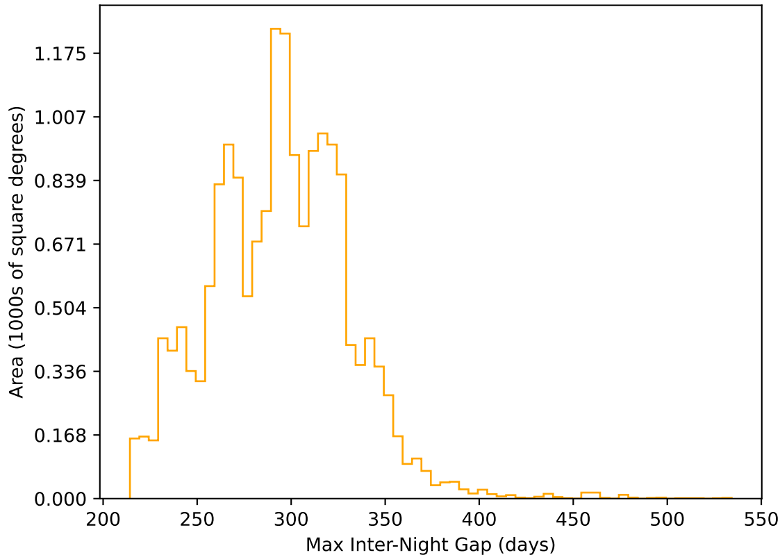
too_elab_r8_d2_ugrizy_v3.4_10yrs WFD r band: Max Inter-Night Gap
