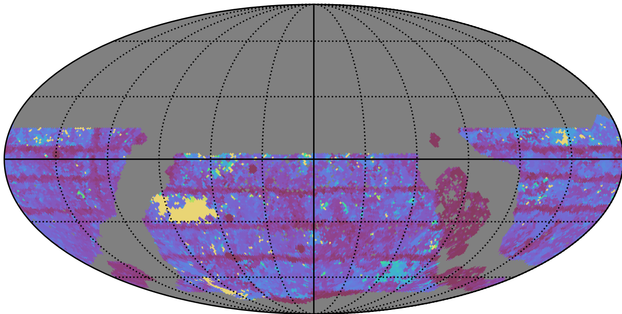
too_elab_r8_d2_ugrizy_v3.4_10yrs WFD i band: Max Inter-Night Gap
