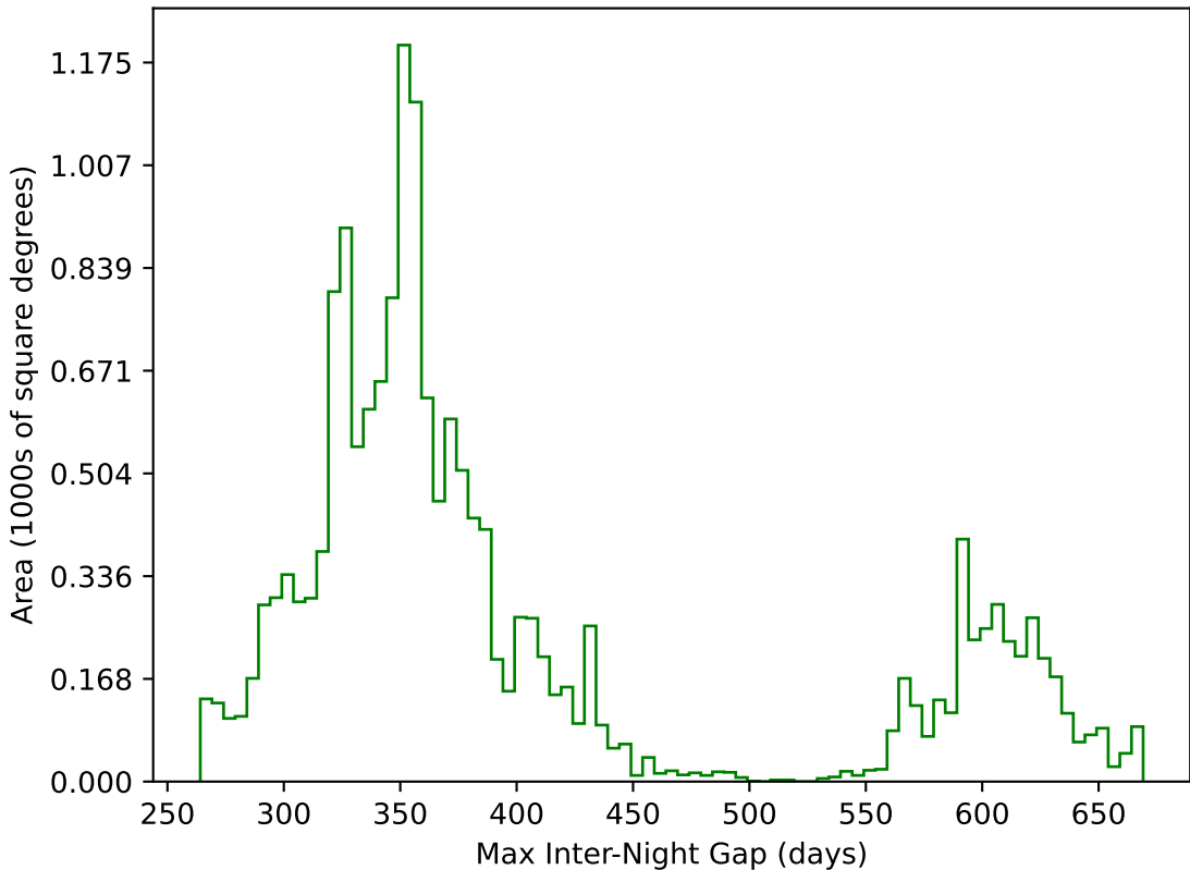
too_elab_r8_d2_ugrizy_v3.4_10yrs WFD g band: Max Inter-Night Gap
