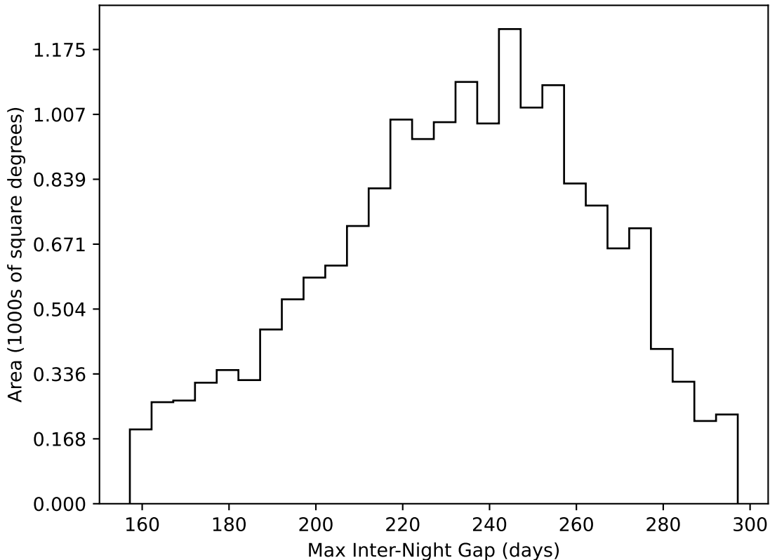
too_elab_r8_d2_ugrizy_v3.4_10yrs WFD all bands: Max Inter-Night Gap
