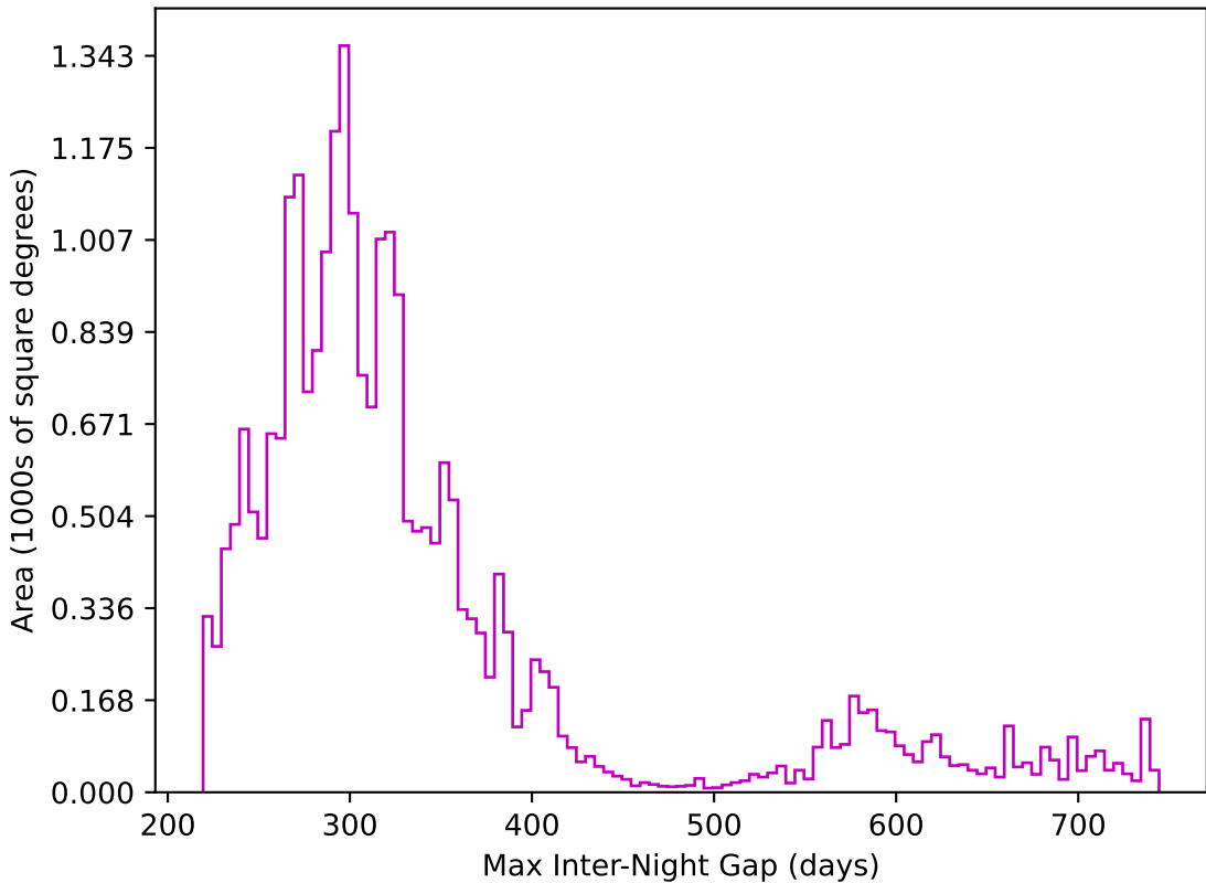
too_elab_r8_d2_ugrizy_v3.4_10yrs All sky z band: Max Inter-Night Gap
