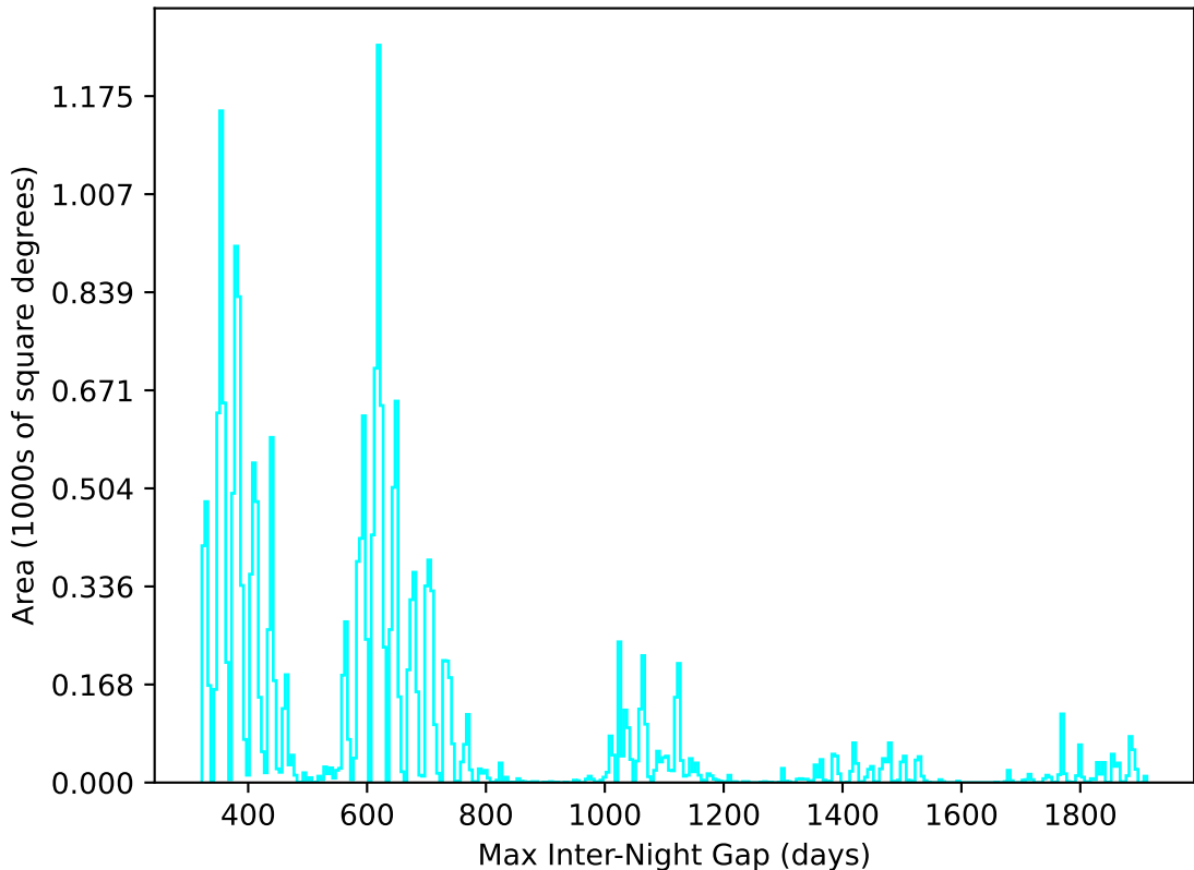
too_elab_r8_d2_ugrizy_v3.4_10yrs All sky u band: Max Inter-Night Gap
