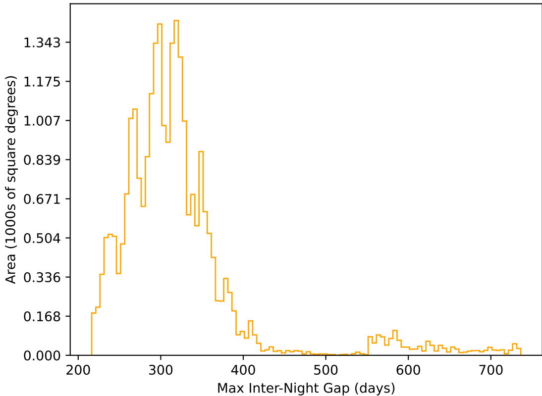
too_elab_r8_d2_ugrizy_v3.4_10yrs All sky r band: Max Inter-Night Gap
