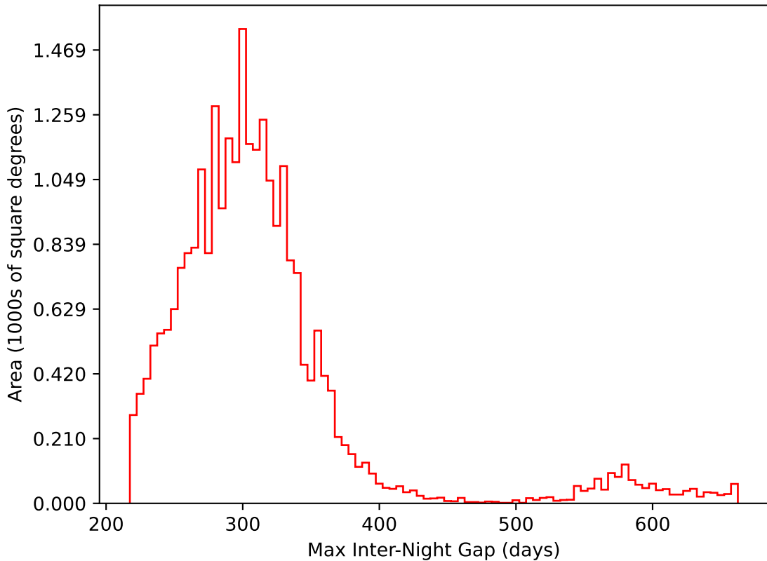
too_elab_r8_d2_ugrizy_v3.4_10yrs All sky i band: Max Inter-Night Gap
