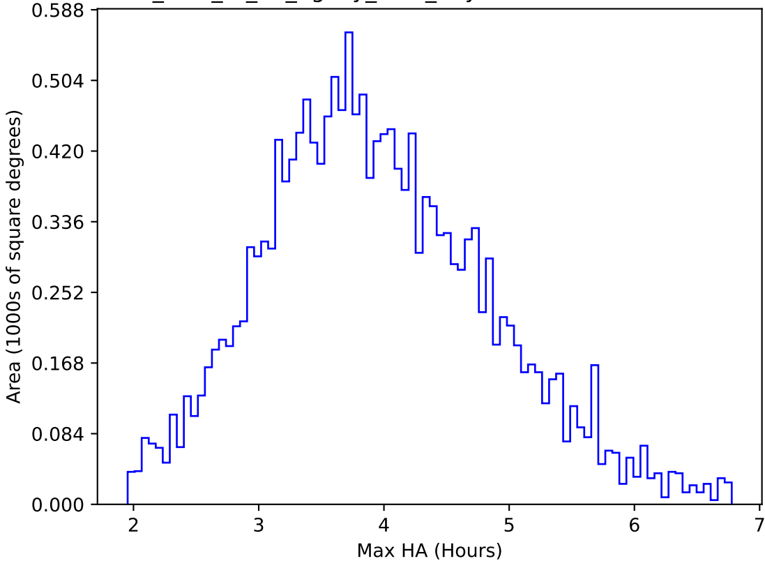
too_elab_r8_d2_ugrizy_v3.4_10yrs WFD u band: Max HA
