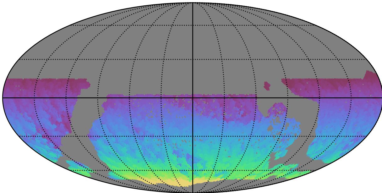
too_elab_r8_d2_ugrizy_v3.4_10yrs WFD all bands: Max HA
