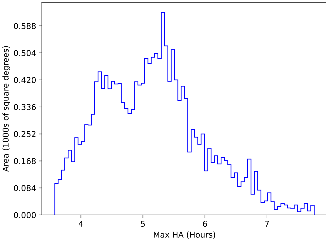
too_elab_r8_d2_ugrizy_v3.4_10yrs WFD all bands: Max HA
