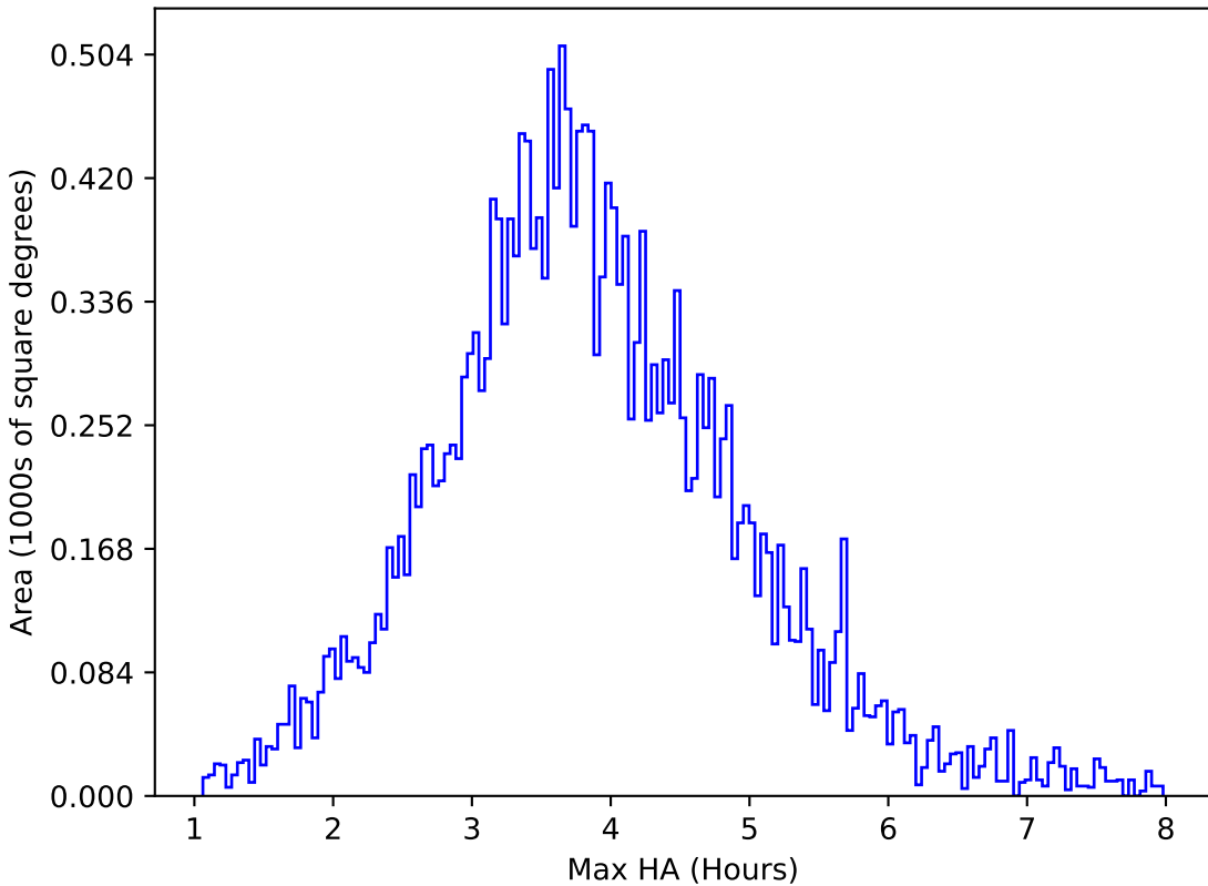
too_elab_r8_d2_ugrizy_v3.4_10yrs All sky u band: Max HA
