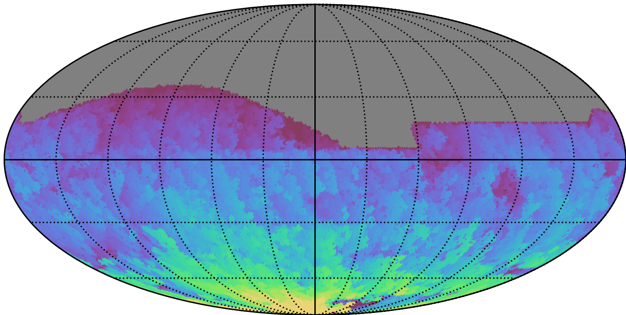
too_elab_r8_d2_ugrizy_v3.4_10yrs All sky r band: Max HA
