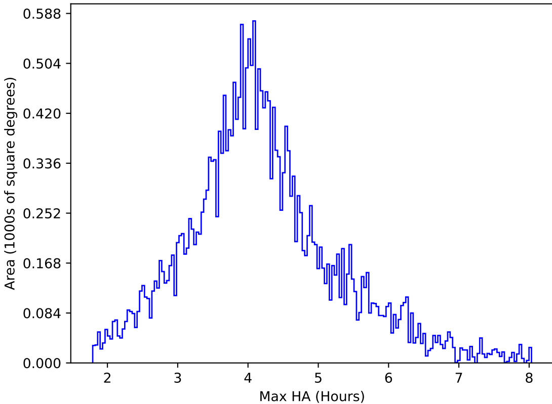
too_elab_r8_d2_ugrizy_v3.4_10yrs All sky r band: Max HA
