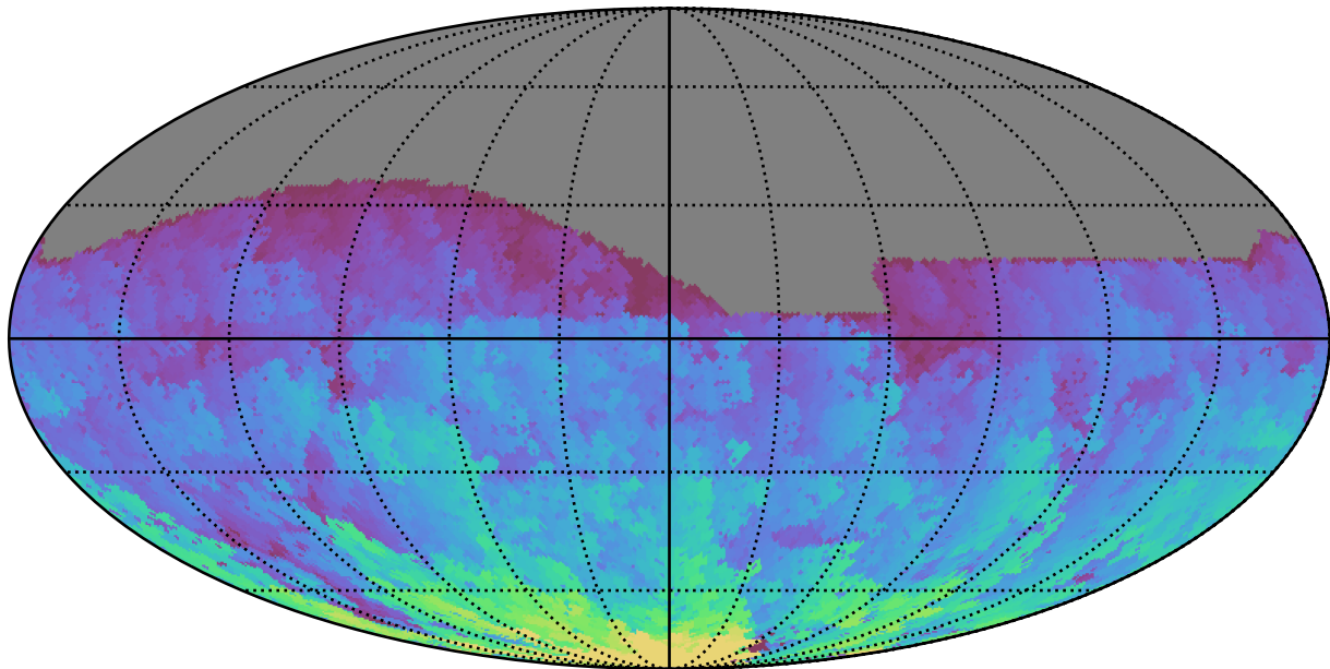
too_elab_r8_d2_ugrizy_v3.4_10yrs All sky g band: Max HA
