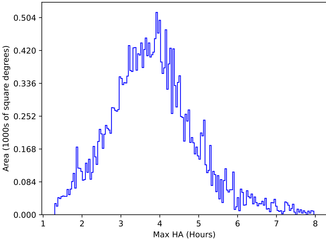
too_elab_r8_d2_ugrizy_v3.4_10yrs All sky g band: Max HA
