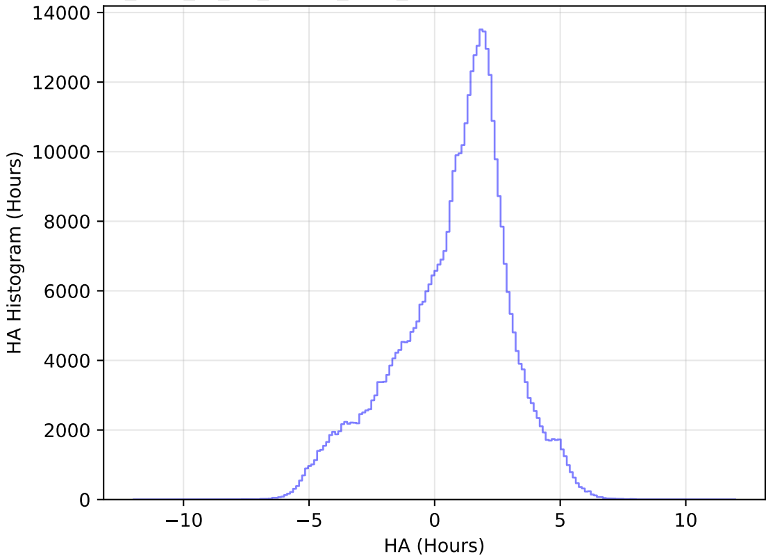
too_elab_r8_d2_ugrizy_v3.4_10yrs WFD z band: HA Histogram
