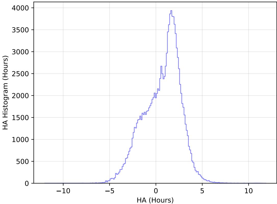
too_elab_r8_d2_ugrizy_v3.4_10yrs WFD u band: HA Histogram
