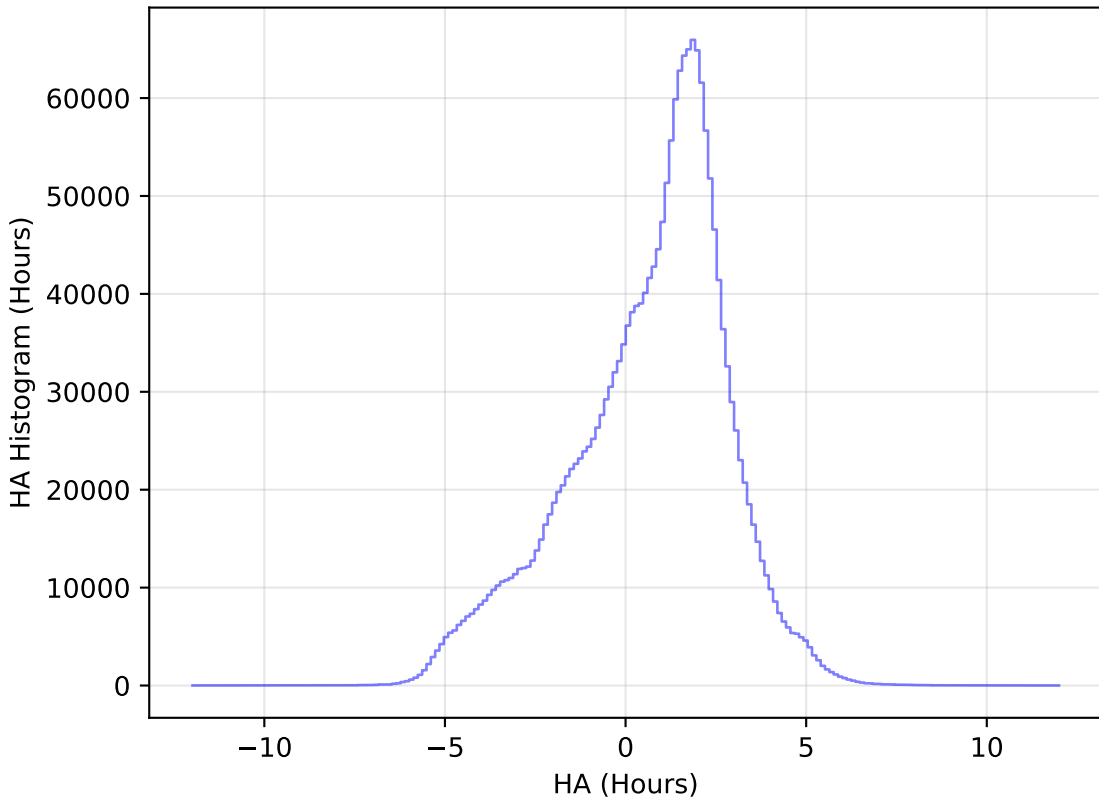
too_elab_r8_d2_ugrizy_v3.4_10yrs WFD all bands: HA Histogram
