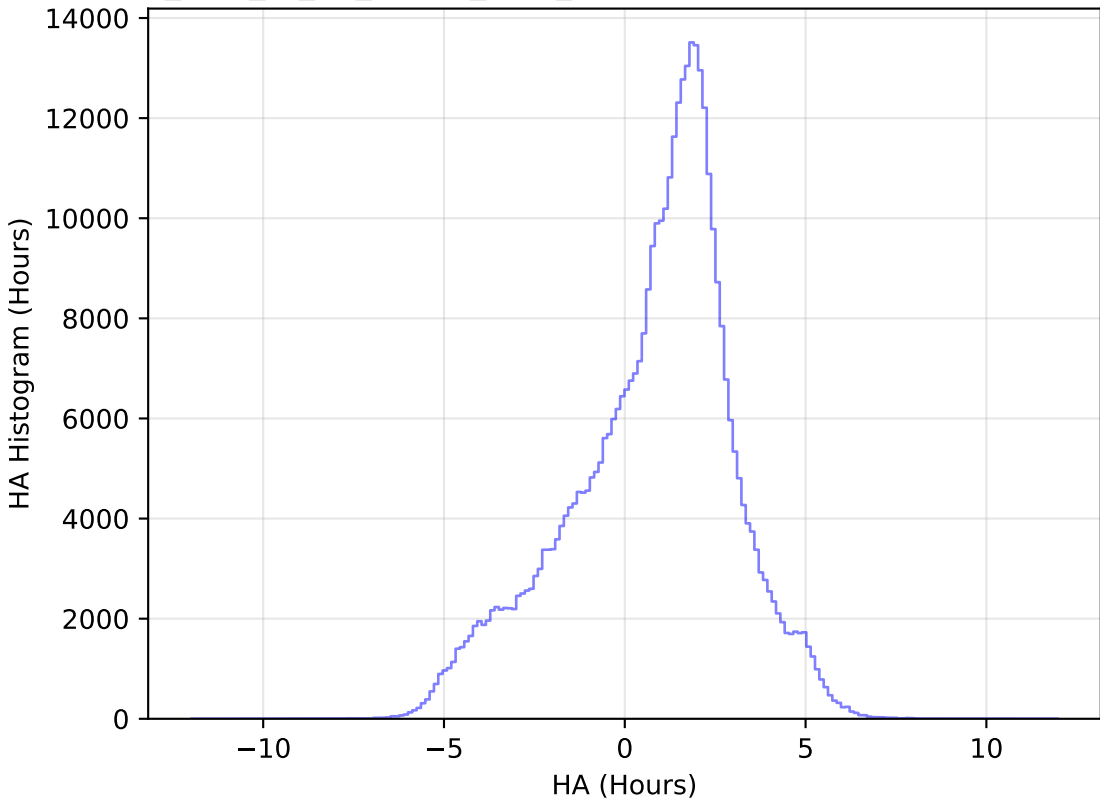
too_elab_r8_d2_ugrizy_v3.4_10yrs All sky z band: HA Histogram
