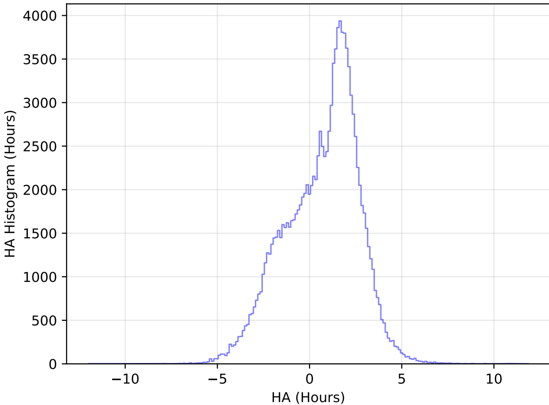
too_elab_r8_d2_ugrizy_v3.4_10yrs All sky u band: HA Histogram
