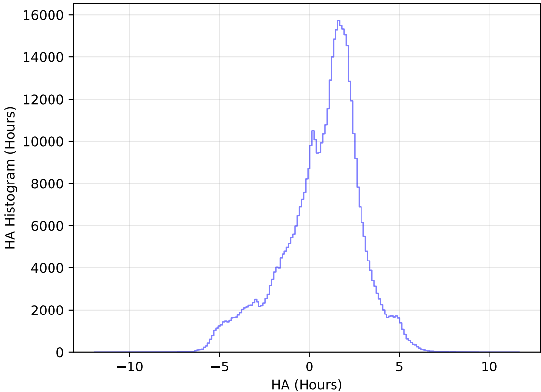
too_elab_r8_d2_ugrizy_v3.4_10yrs All sky i band: HA Histogram
