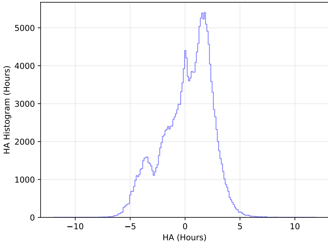
too_elab_r8_d2_ugrizy_v3.4_10yrs All sky g band: HA Histogram
