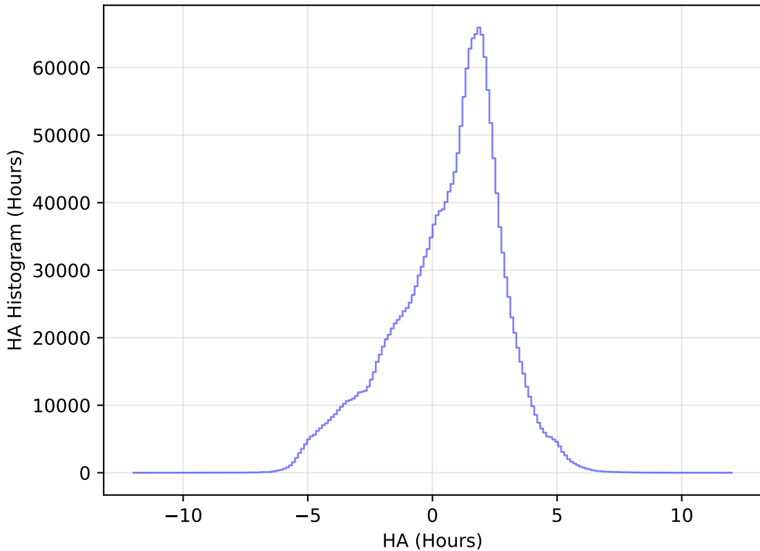
too_elab_r8_d2_ugrizy_v3.4_10yrs All sky all bands: HA Histogram
