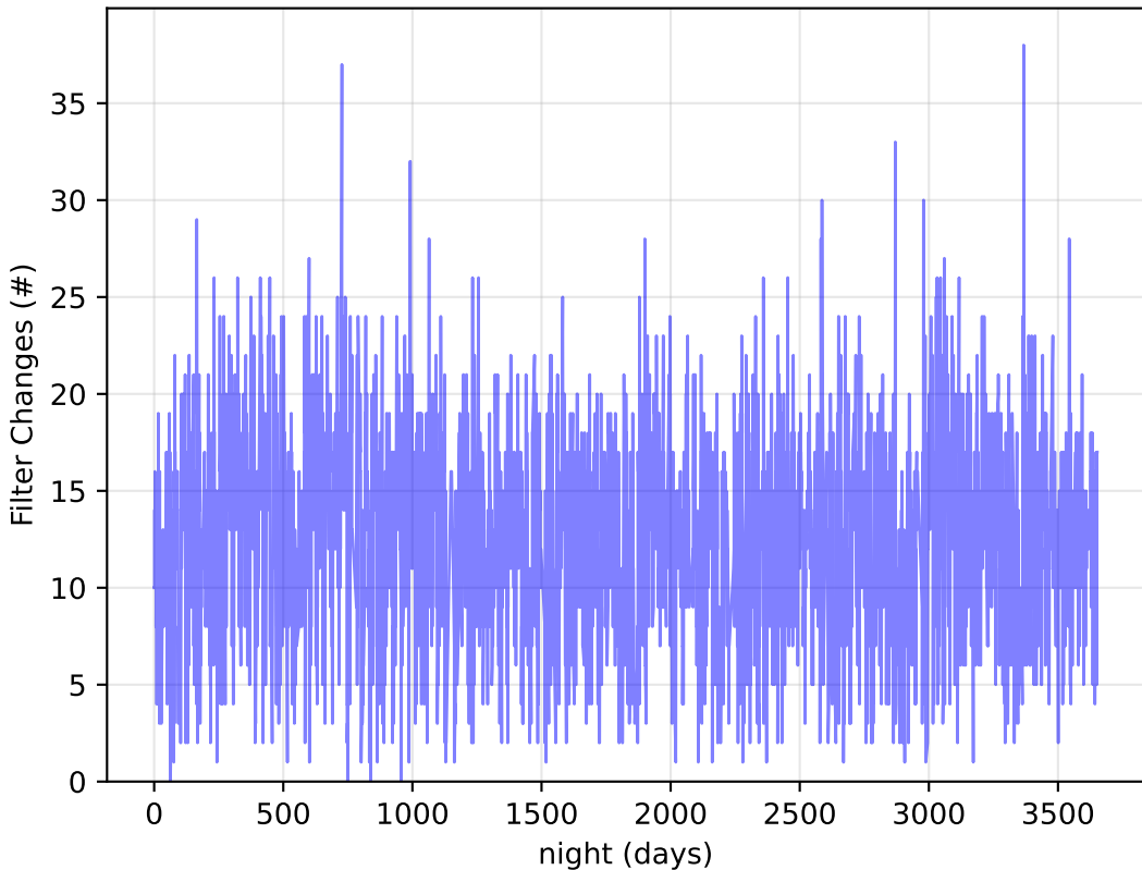
too_elab_r8_d2_ugrizy_v3.4_10yrs Per Night: Filter Changes
