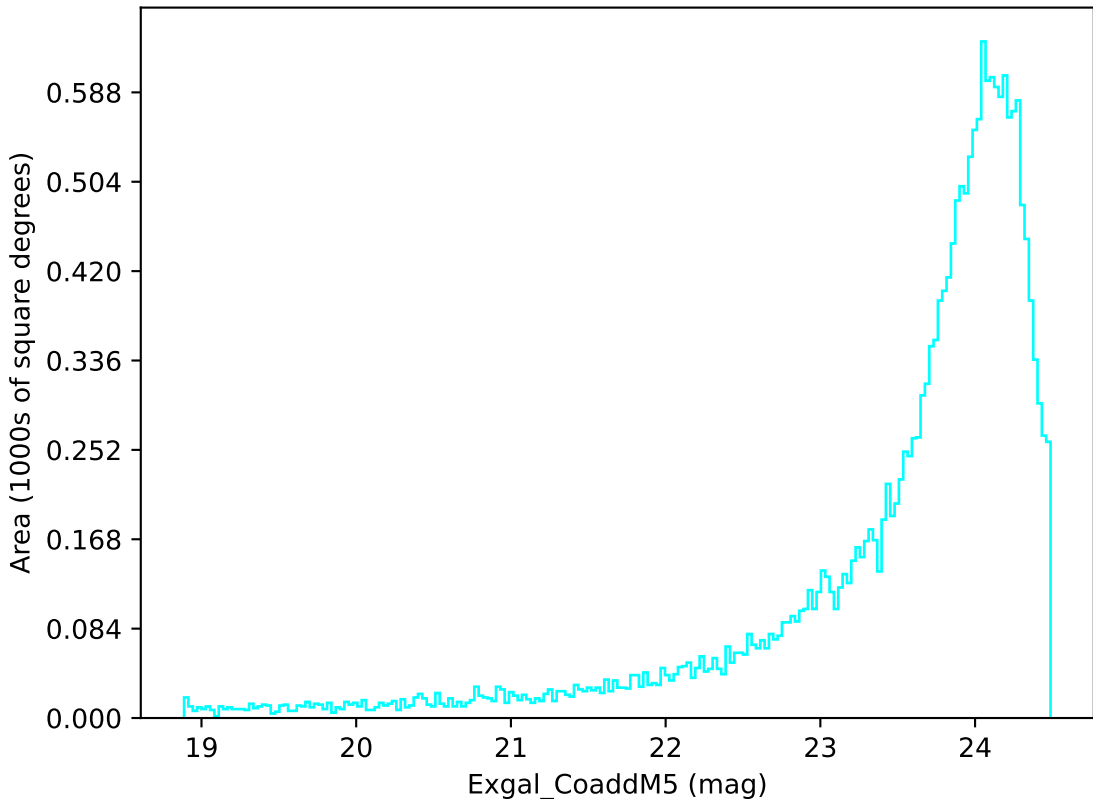
too_elab_r8_d2_ugrizy_v3.4_10yrs Yr 1 u band: Exgal_CoaddM5
