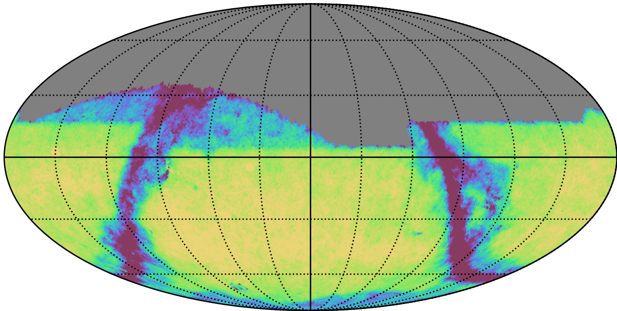
too_elab_r8_d2_ugrizy_v3.4_10yrs Yr 1 i band: Exgal_CoaddM5
