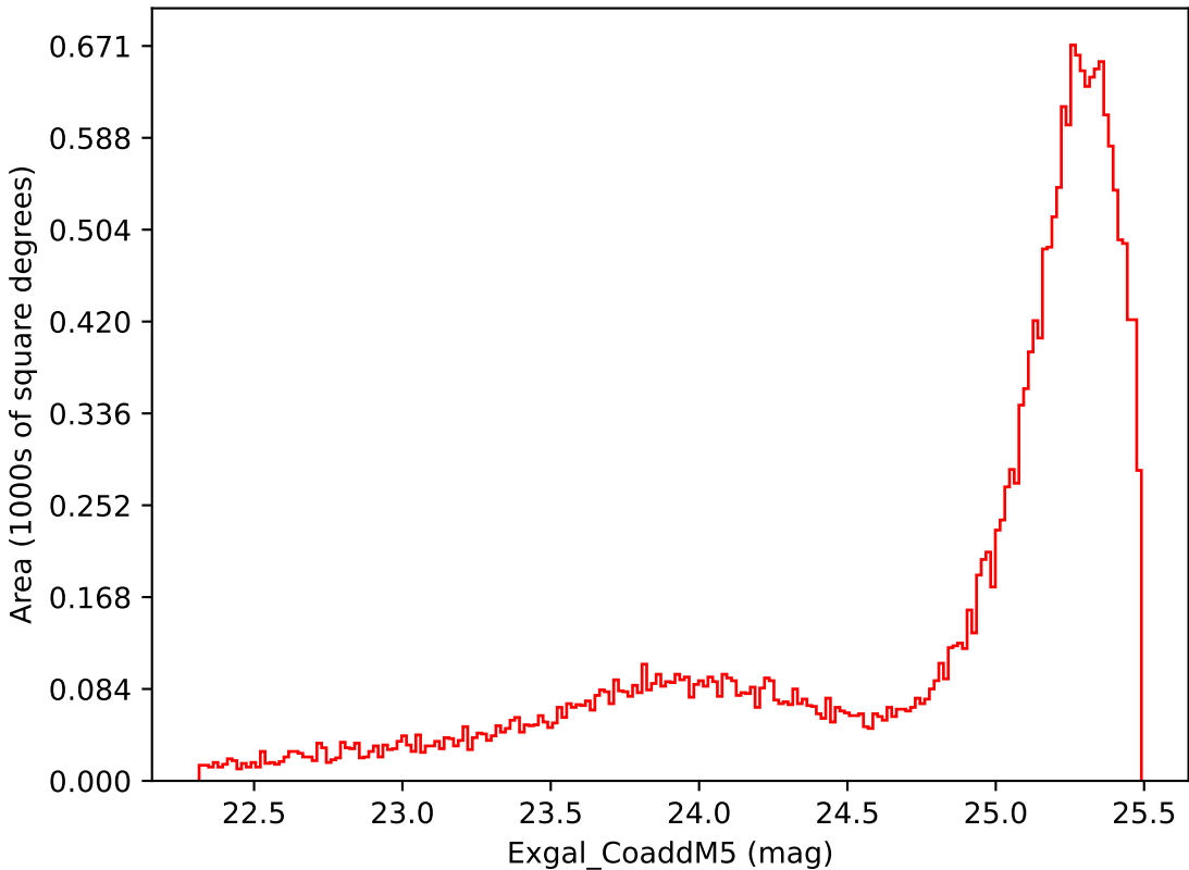
too_elab_r8_d2_ugrizy_v3.4_10yrs Yr 1 i band: Exgal_CoaddM5
