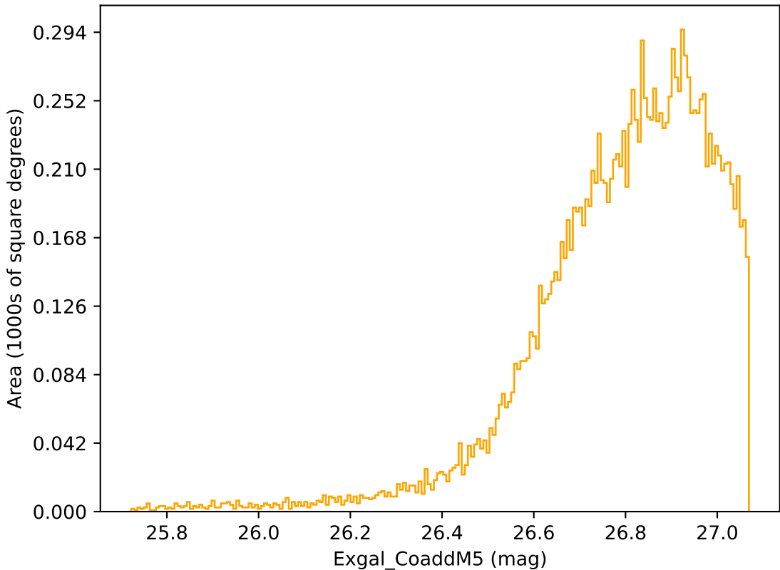
too_elab_r8_d2_ugrizy_v3.4_10yrs WFD r band: Exgal_CoaddM5
