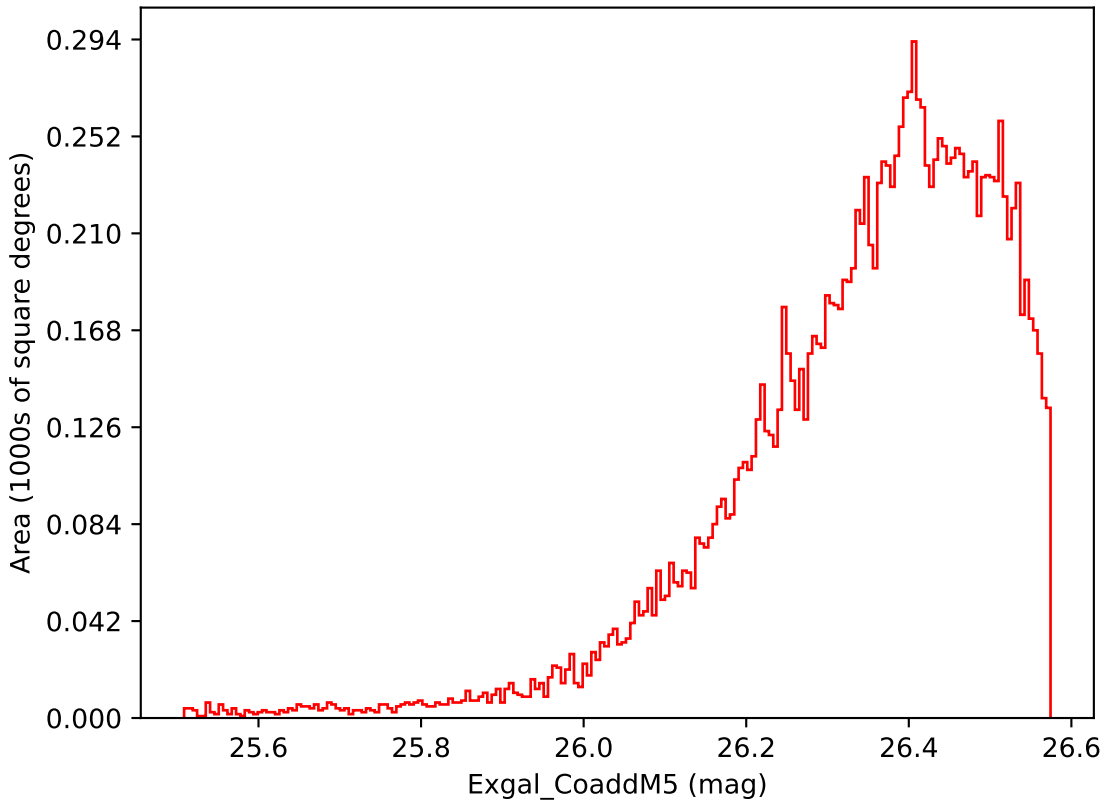
too_elab_r8_d2_ugrizy_v3.4_10yrs WFD i band: Exgal_CoaddM5
