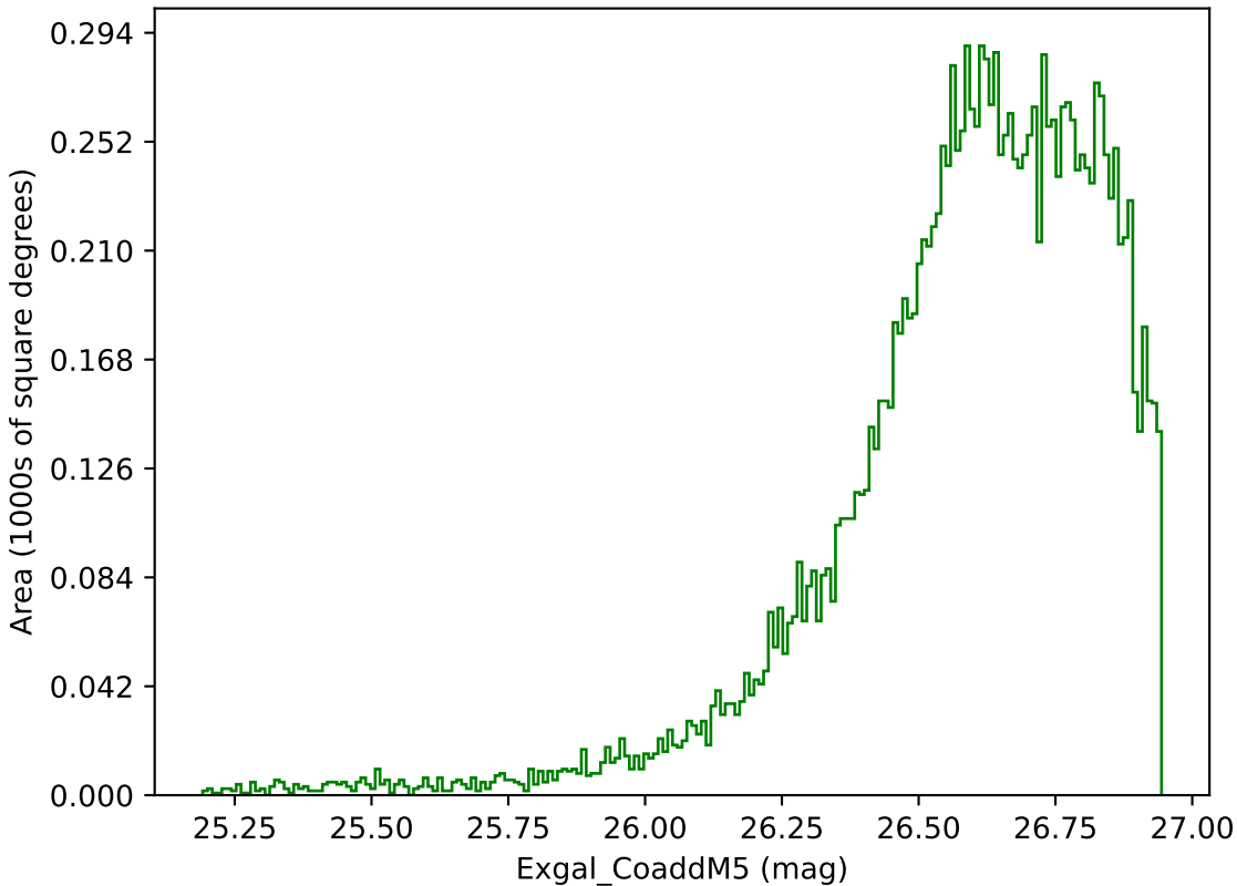
too_elab_r8_d2_ugrizy_v3.4_10yrs WFD g band: Exgal_CoaddM5
