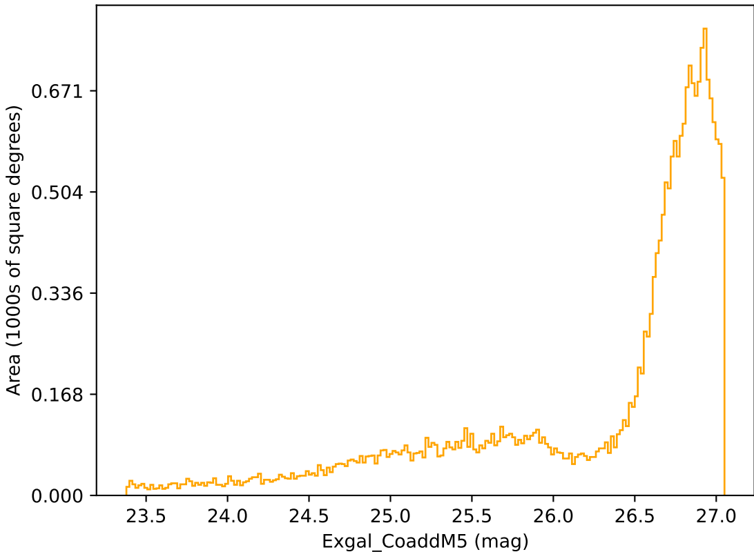
too_elab_r8_d2_ugrizy_v3.4_10yrs All sky r band: Exgal_CoaddM5
