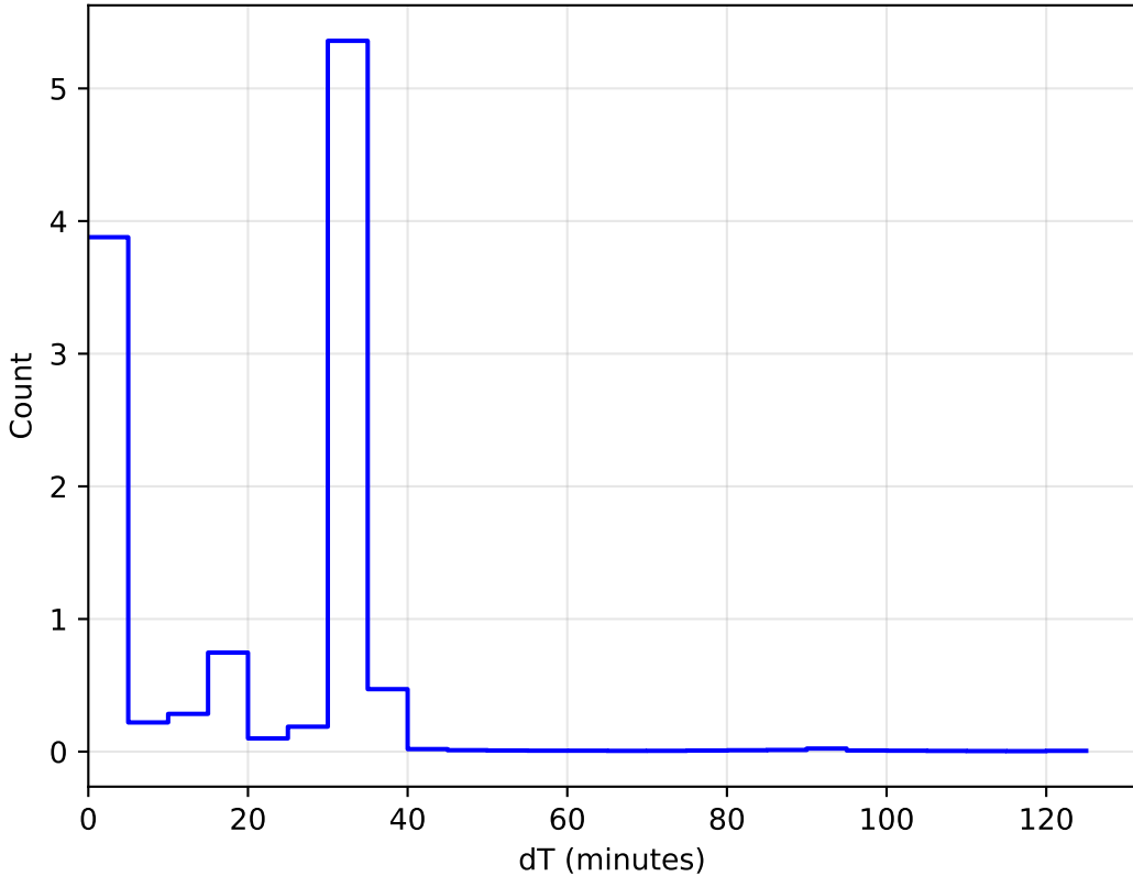
too_elab_r8_d2_ugrizy_v3.4_10yrs WFD: DeltaT Histogram 1e6
