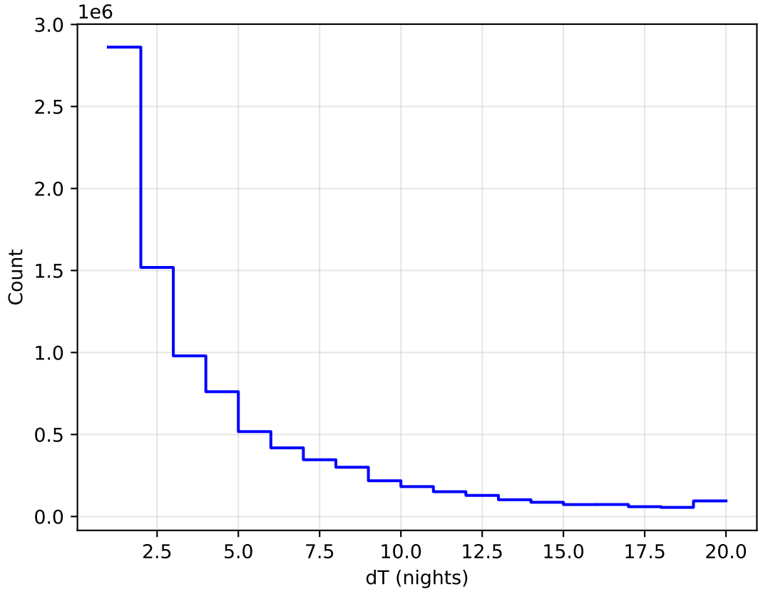
too_elab_r8_d2_ugrizy_v3.4_10yrs All sky all bands: DeltaNight Histogram
