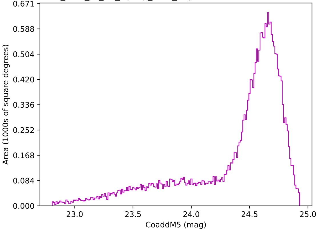
too_elab_r8_d2_ugrizy_v3.4_10yrs Yr 1 z band: CoaddM5
