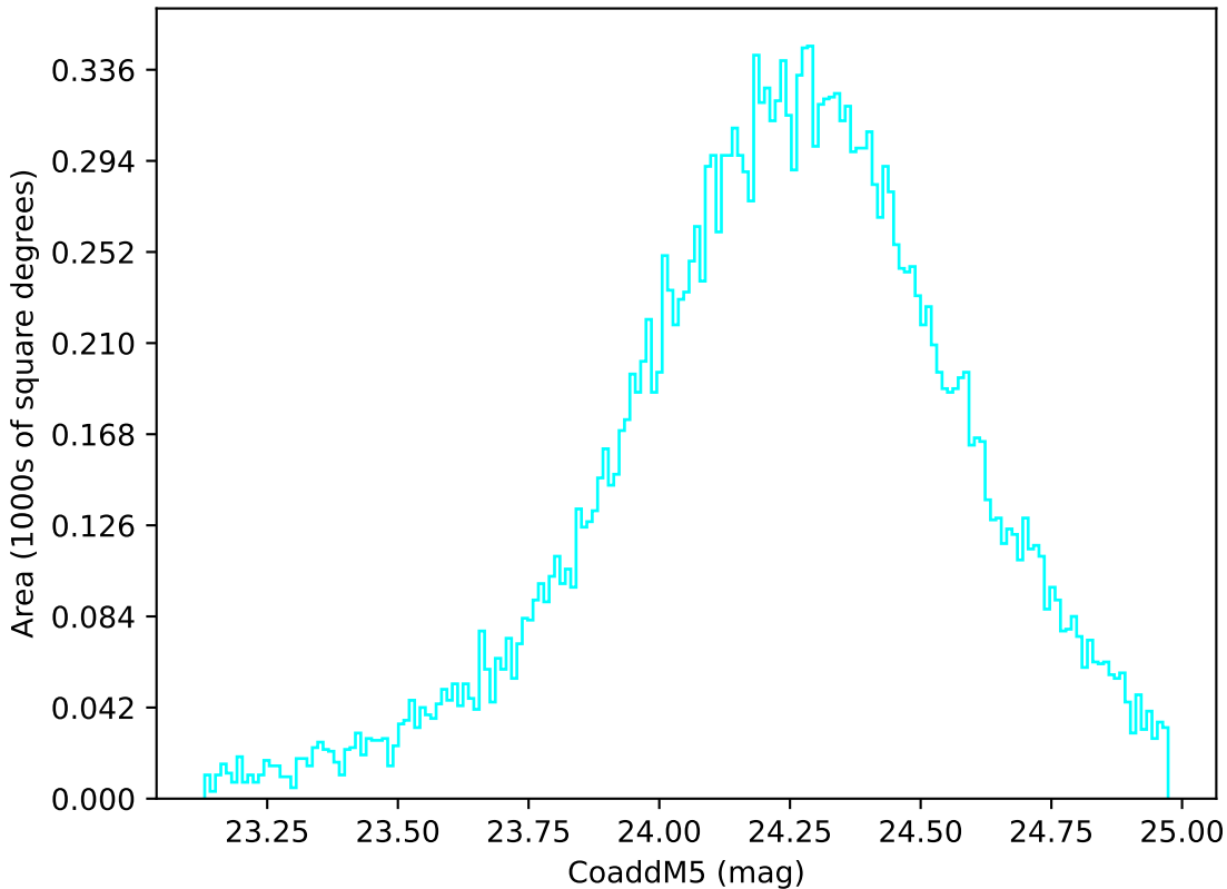
too_elab_r8_d2_ugrizy_v3.4_10yrs Yr 1 u band: CoaddM5
