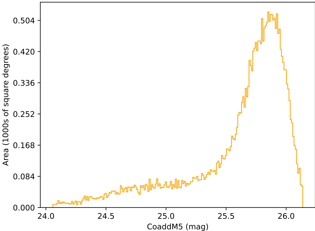
too_elab_r8_d2_ugrizy_v3.4_10yrs Yr 1 r band: CoaddM5
