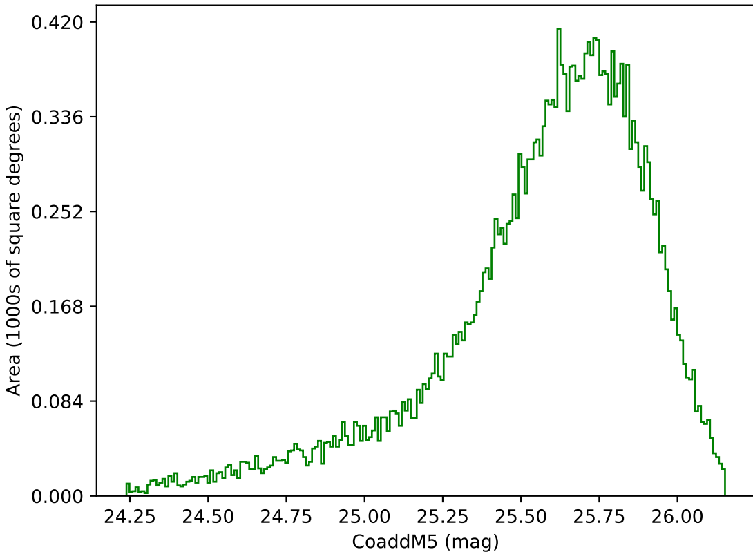
too_elab_r8_d2_ugrizy_v3.4_10yrs Yr 1 g band: CoaddM5
